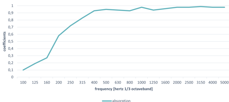
Jackson coefficients NEN-EN-ISO 354:2003
