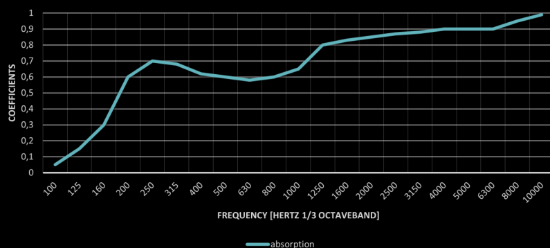
Dylan coefficients NEN-EN-ISO 354:2003
