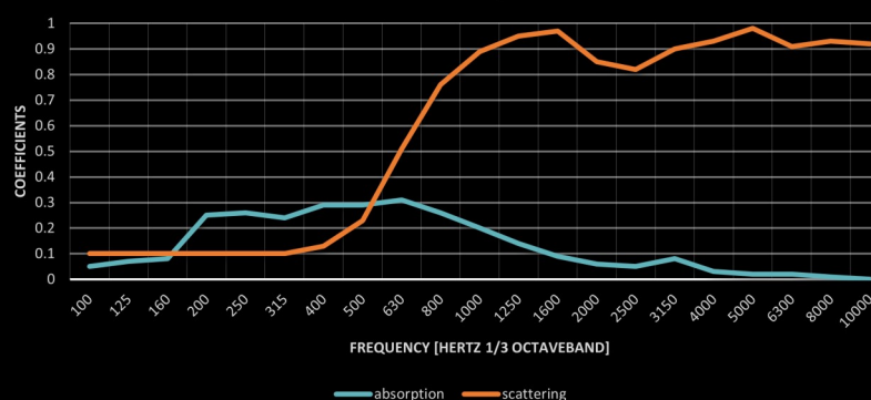
KEYS coefficients NEN-EN-ISO 354:2003 / ISO 17497-2
