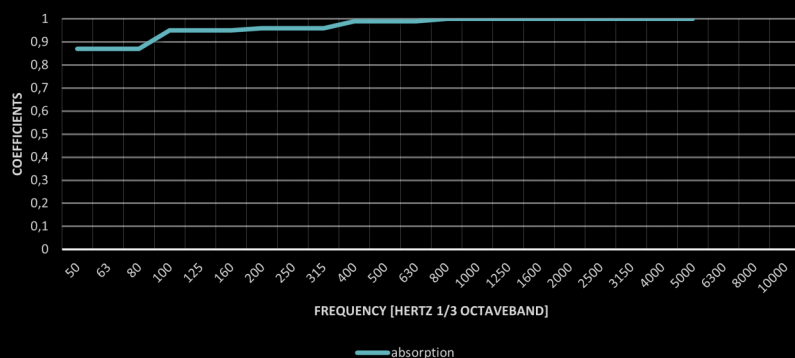
Parton coefficients NEN-EN-ISO 354:2003
