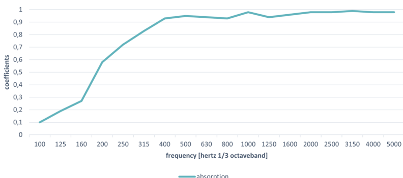
Franklin coefficients NEN-EN-ISO 354:2003
